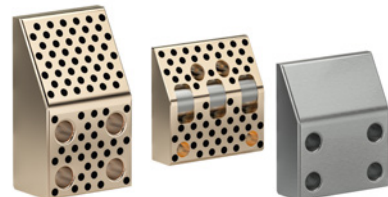
Cam stroke plates with/without roller
